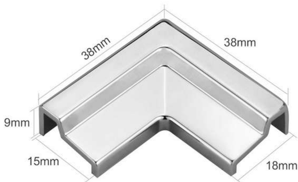
AS101-90 CORNER CONNECTOR
